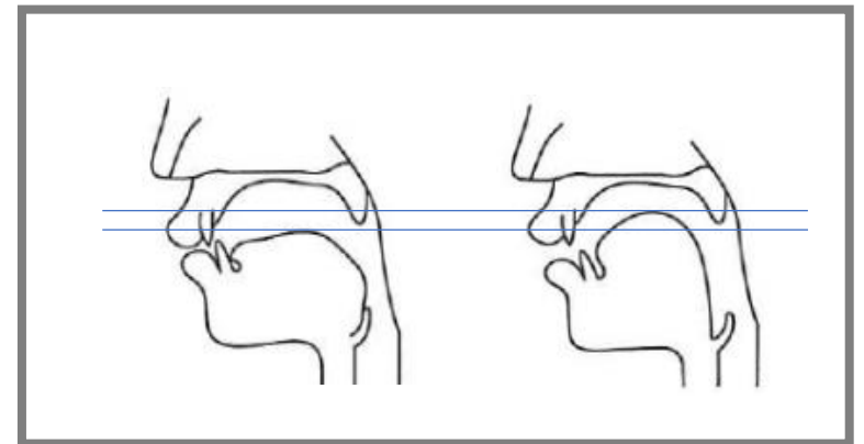
図3 [ϕ]と[h]
